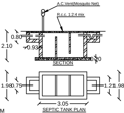
SEPTIC TANK PLAN
