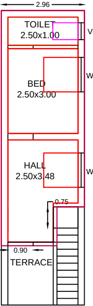
PROPOSED FIRST FLOOR PLAN
