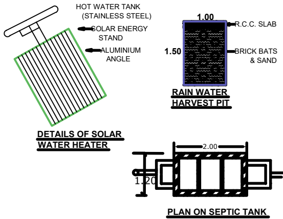
PLAN ON SEPTIC TANK
