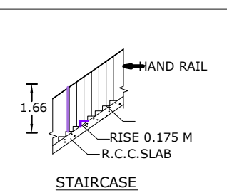
STAIRCASE
