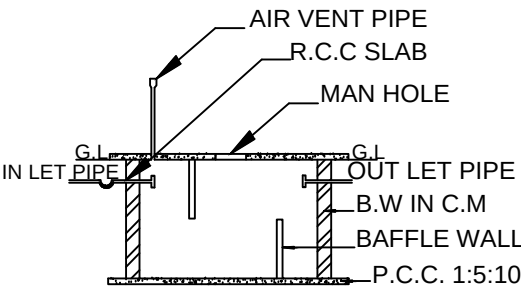
SECTION ON SEPTIC TANK
