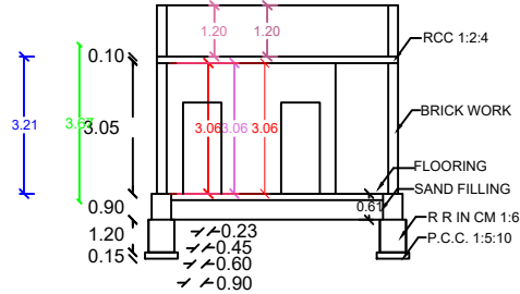
SECTION AB
