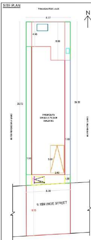
SITE PLAN
