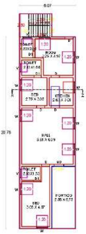
PLAN
