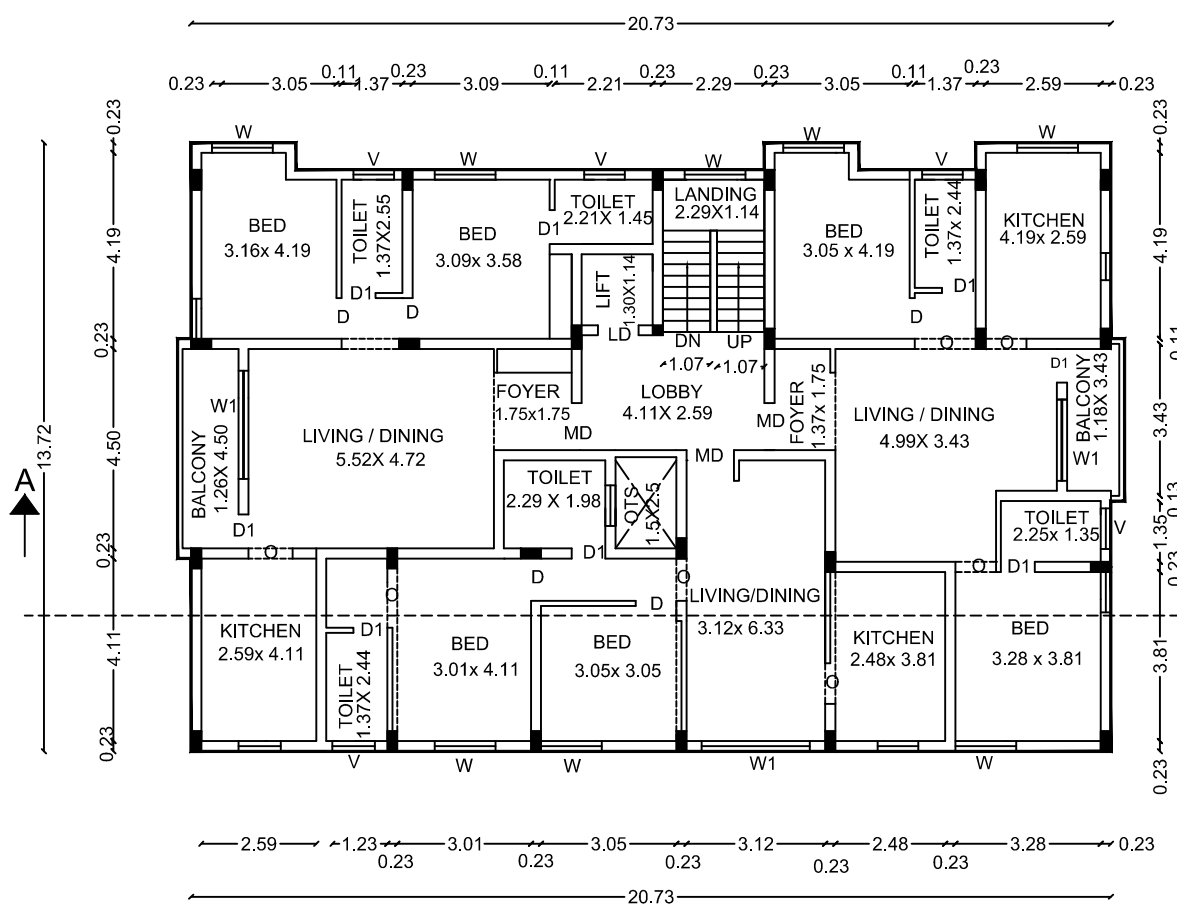
TYPICAL FLOOR PLAN (1ST, 2ND)
