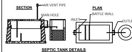
SEPTIC TANK DETAILS
