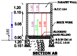
SECTION AB
