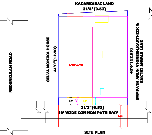
SCALE 1:100
