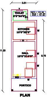
PLAN
