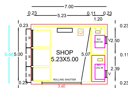
PRO GROUND FLOOR COMMERCIAL PLAN
