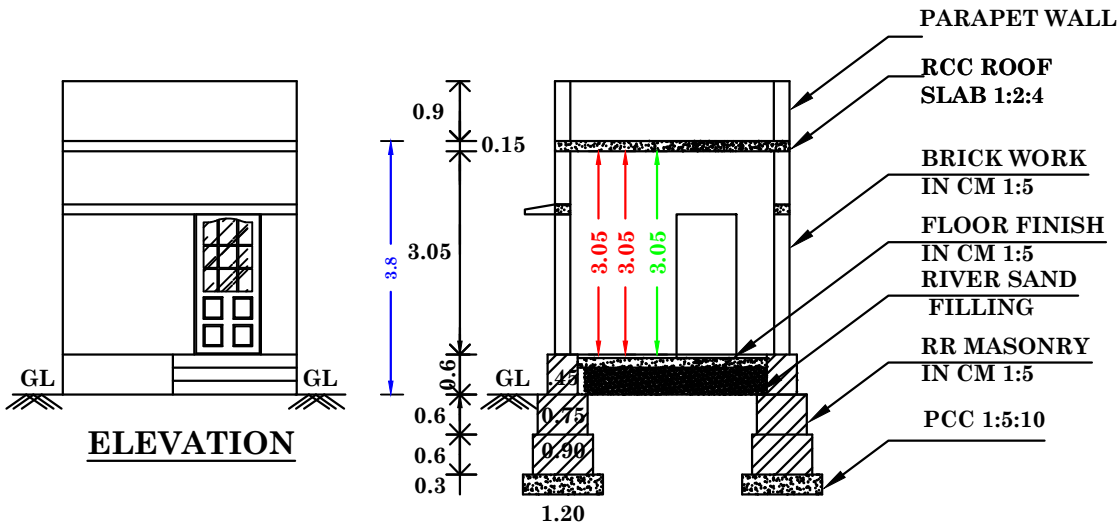
SECTION ON AA1
