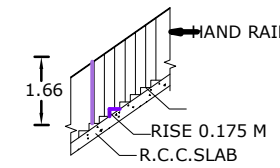
STAIRCASE
