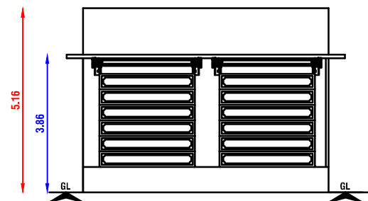
FRONT ELEVATION
