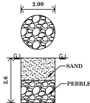
RAINWATER HARVESTING
