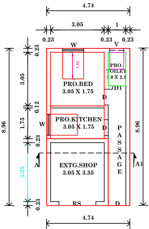
EXISTING AND PROPOSED GROUND FLOOR PLAN
