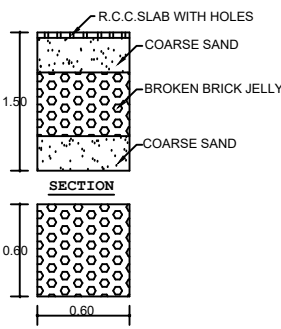
WASTE WATER FROM WASH BASIN AND BATHROOM ARE RECHARGED AND RECYCLED AND TO BE CONNECTED WITH R.W.H. PIT.
