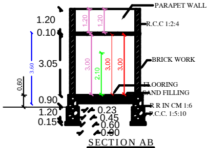
SECTION AB
