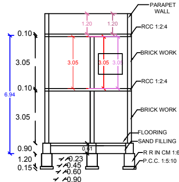
SECTION AB
