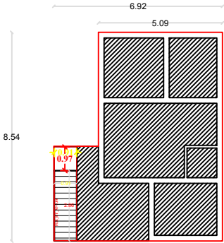
EXG.GROUND FLOOR PLAN
