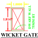
WICKET GATE
