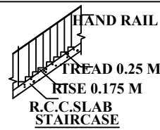
R.C.C.SLAB STAIRCASE
