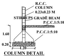
COLUMN DETAIL
