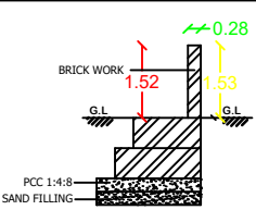
SECTION OF COMPOUND WALL
