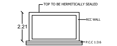
SECTION ON U.G.SUMP
