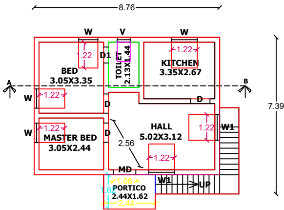
TYPICAL_FLOOR_PLAN=1
