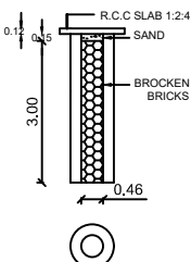
PERCOLATION PIT
