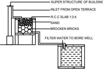
DETAILS OF FILTER BED & WELL
