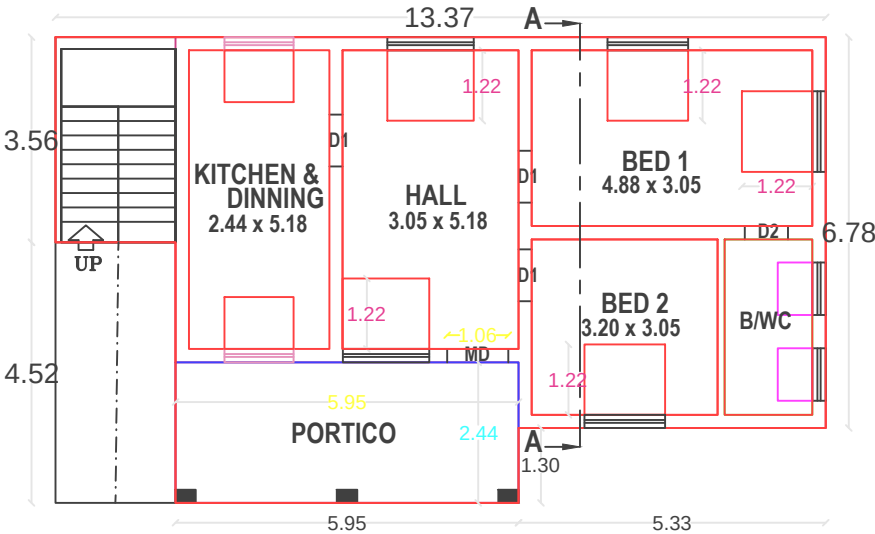
PLAN - GROUND FLOOR (PROPOSED)
