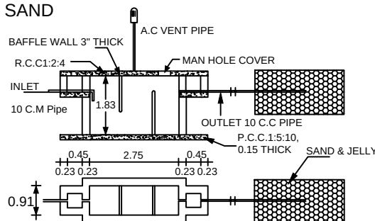
SEPTIC TANK AND TRECH
