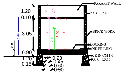
SECTION AB
