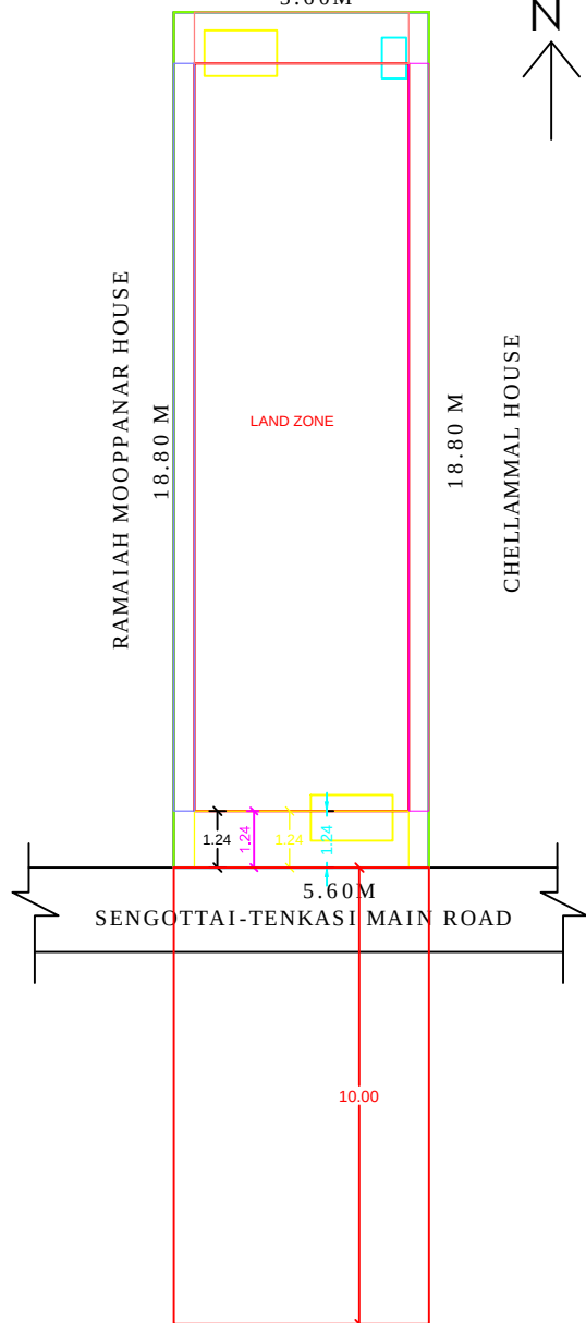
SITE PLAN
