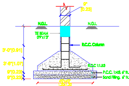
FOUNDATION DETAIL
