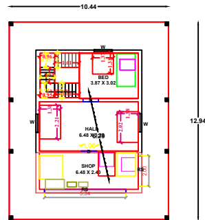
GROUND FLOOR HOUSE & SHOP PLAN
