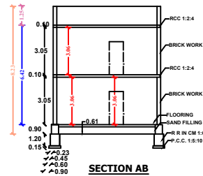
SECTION AB
