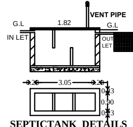
SEPTICTANK DETAILS
