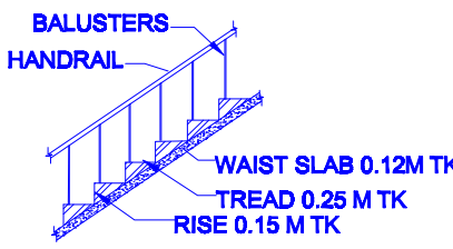
STAIRCASE DETAILS
