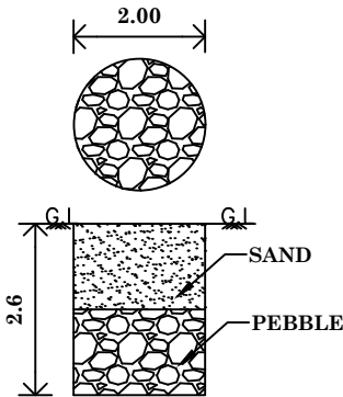
RAINWATER HARVESTING
