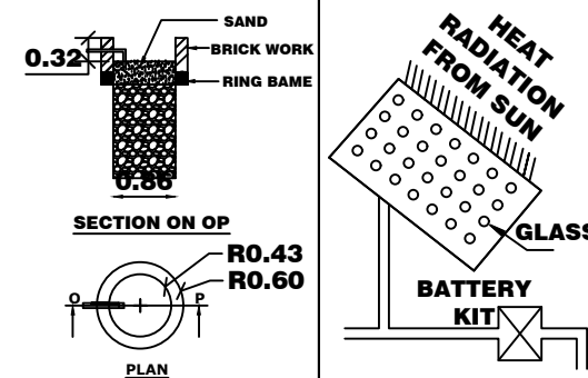
RAIN WATER PIT
