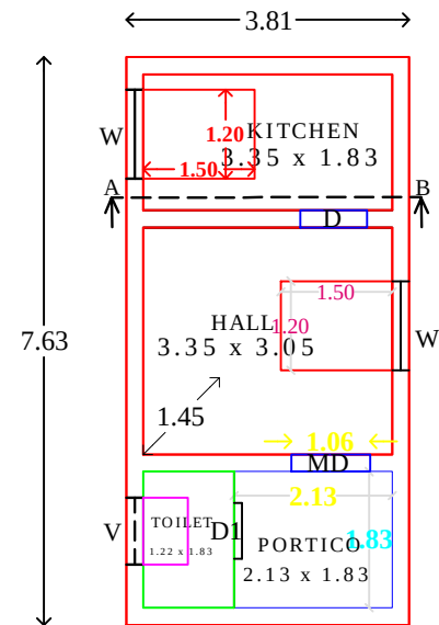
PLAN
