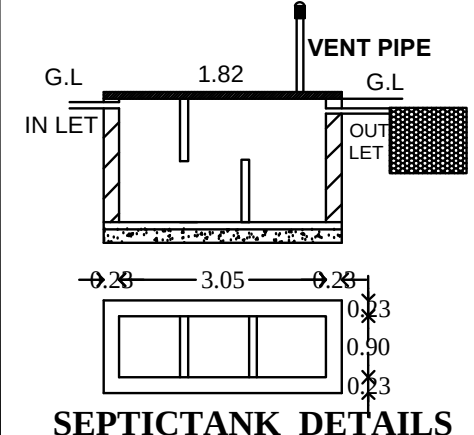
SEPTICTANK DETAILS
