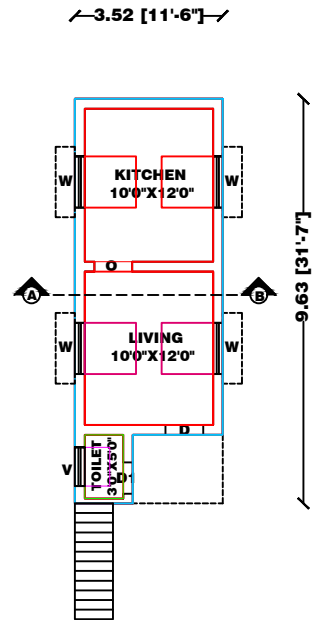
PLAN
