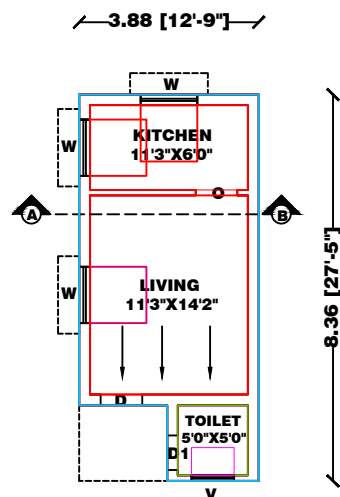
PLAN
