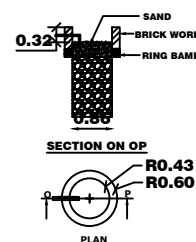
RAIN WATER PIT
