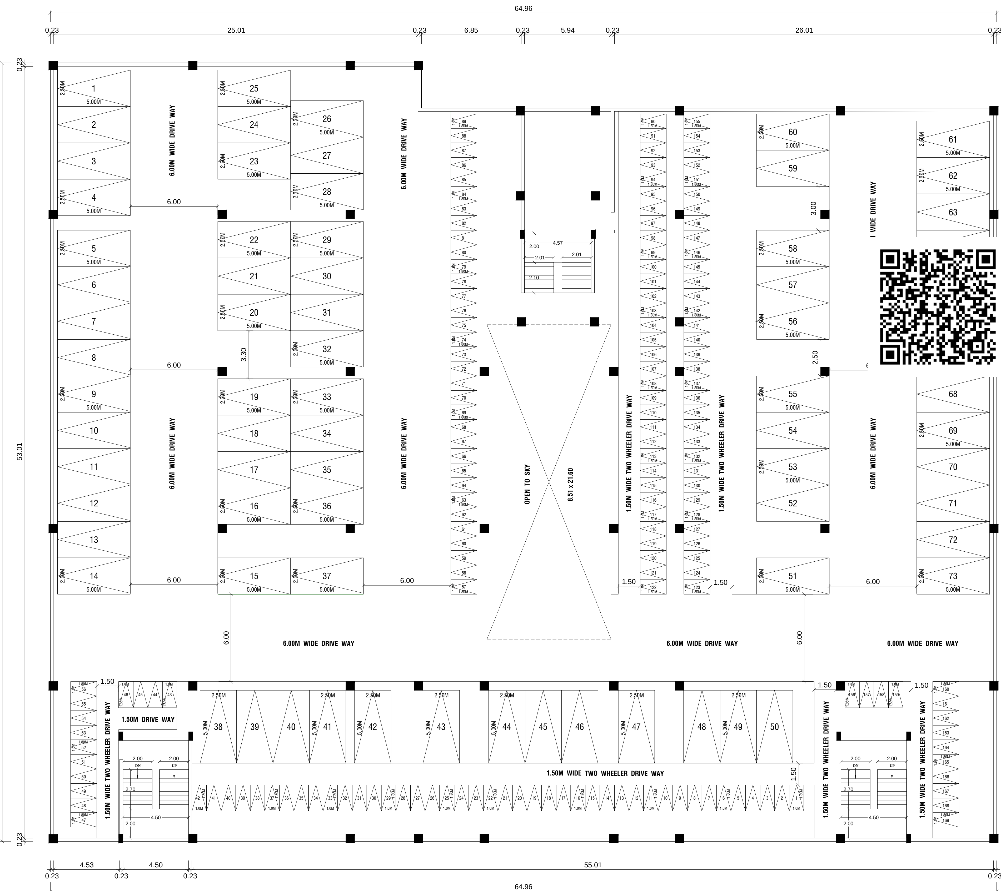
BASEMENT FLOOR PLAN
