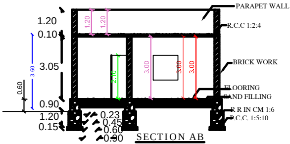
SECTION AB
