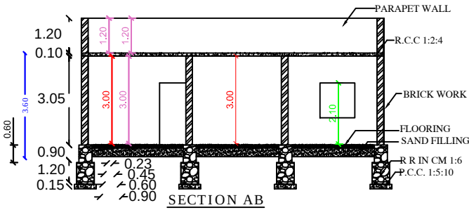
SECTION AB
