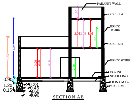
SECTION AB
