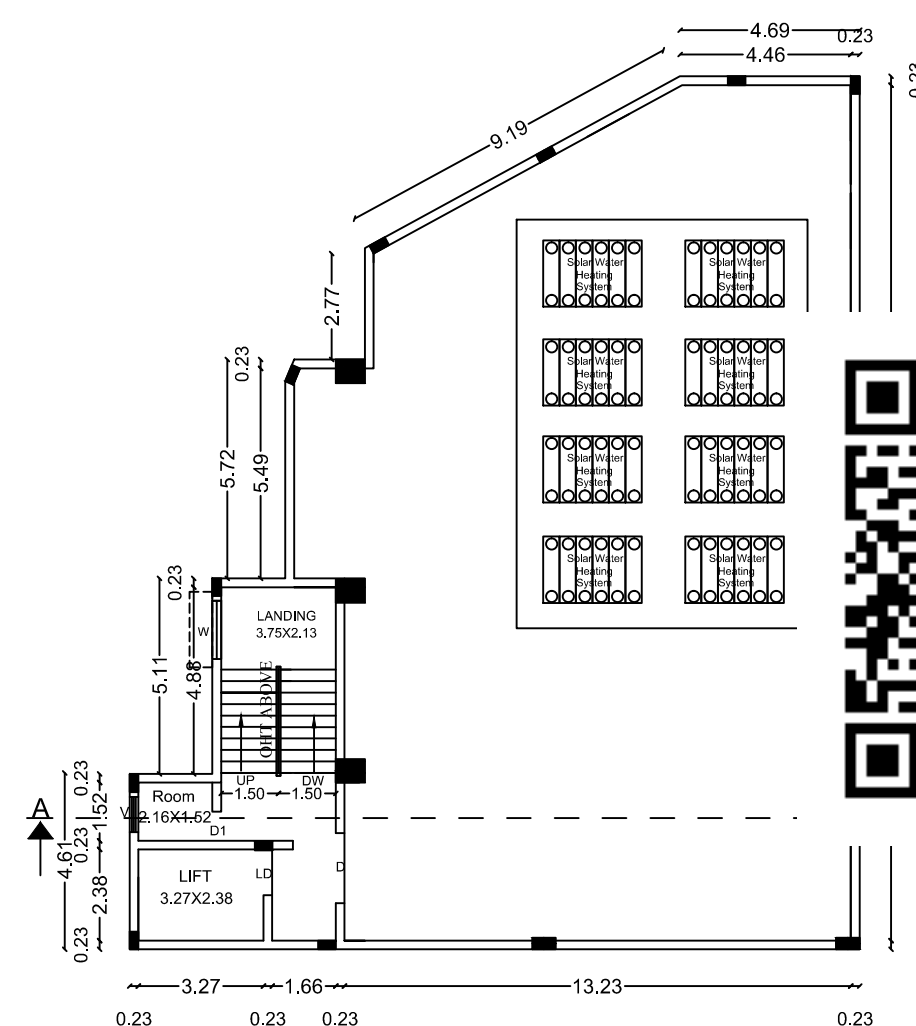
TERRACE FLOOR
