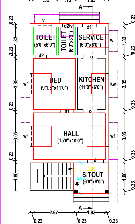
PLAN - RESIDENCE
