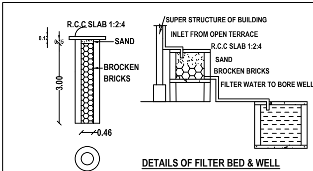
PERCOLATION PIT
