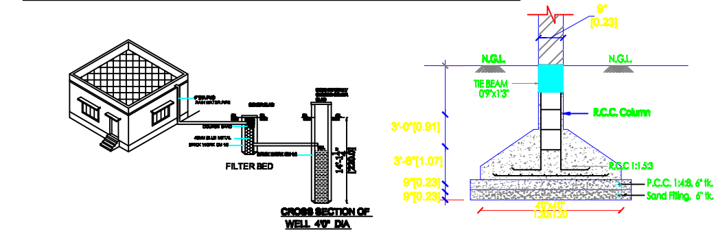
PRO.RAIN WATER SYSTEM
