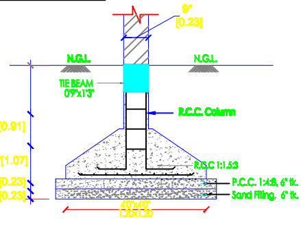
FOUNDATION DETAIL
