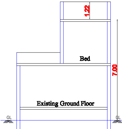
SECTION-B
