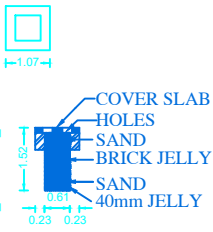
SECTION OF RAIN WATER COLLECTION TANK
