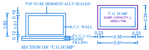
SECTION ON "U.G.SUMP"
