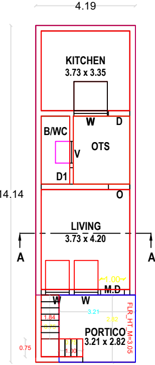
PLAN - GROUND FLOOR
