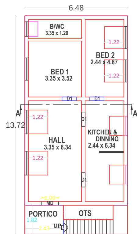
PLAN - GROUND FLOOR ( PROPOSED )
