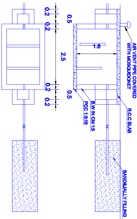
PLAN&SECTION OF SEPTIC TANK TRENCH
