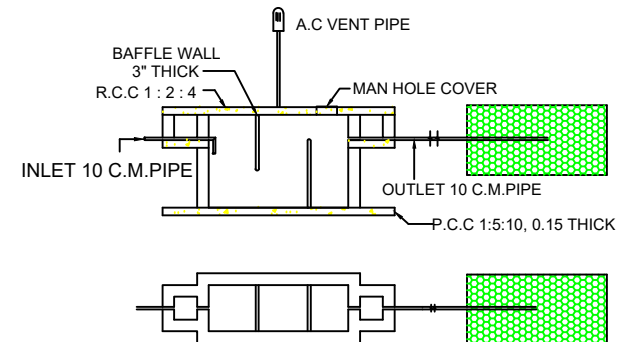
SEPTIC TANK & TRENCH
