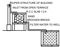
RAINWATER HARVESTING
