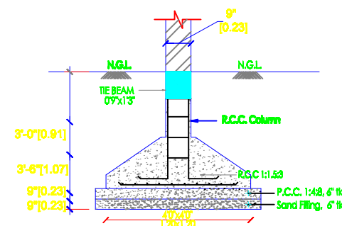
FOUNDATION DETAIL
