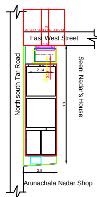
SITE PLAN
