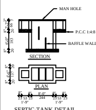
SEPTIC-TANK DETAIL
