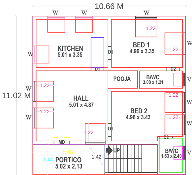
PLAN - GROUND FLOOR (PROPOSED)
