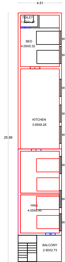
SEC.FLOOR PLAN
