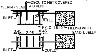
SEPTIC TANK & TRENCH U TRAP PROVISION
