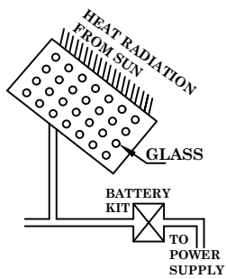
SOLAR SYSTEM
