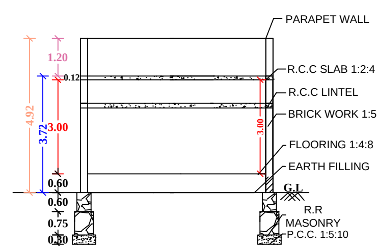
"SECTION "AB"
