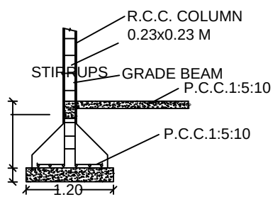
COLUMN DETAIL
