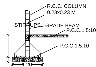
COLUMN DETAIL
