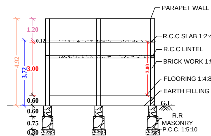
"SECTION "AB"
